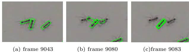
Fig. 2. (a) Three interacting ants are being tracked using independent particle filters. (b) The target with the best likelihood score typically “hijacks” the filters of nearby targets. (c) Resulting tracker failure. We address this problem using an Markov random field motion prior, built on the fly at each time step, that can adequately model these interactions and defeat these failure modes.
